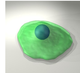
Computational model
