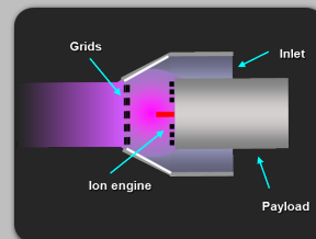
ABIE Air Breathing Ion Engine
