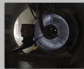
ABIE Air Breathing Ion Engine
